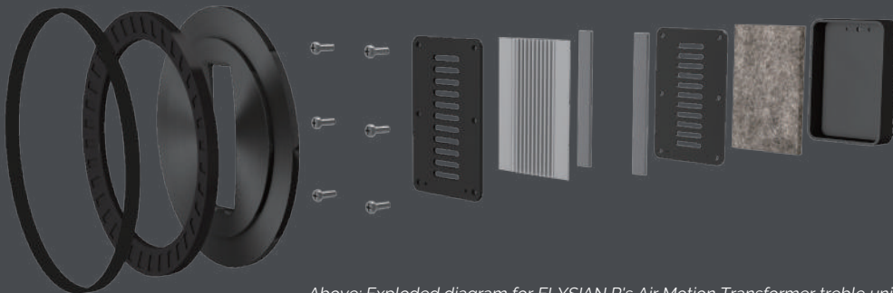
Above: Exploded diagram for ELYSIAN R's Air Motion Transformer treble unit.
